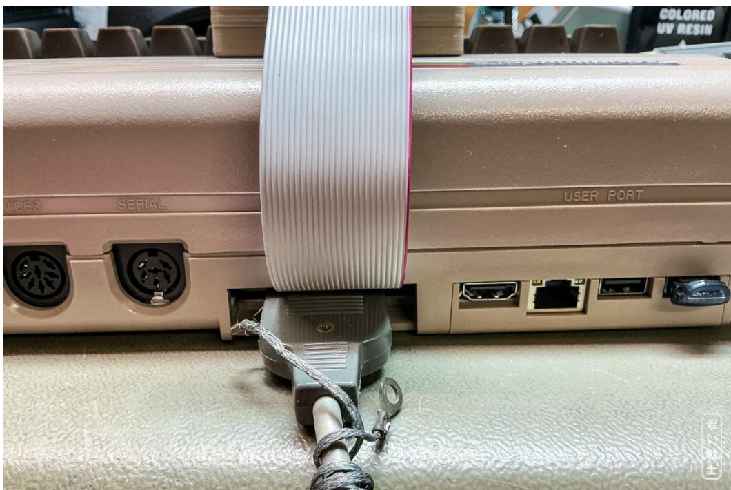
Figure 5: Cassette Port with ribbon cable and Datassette connector
