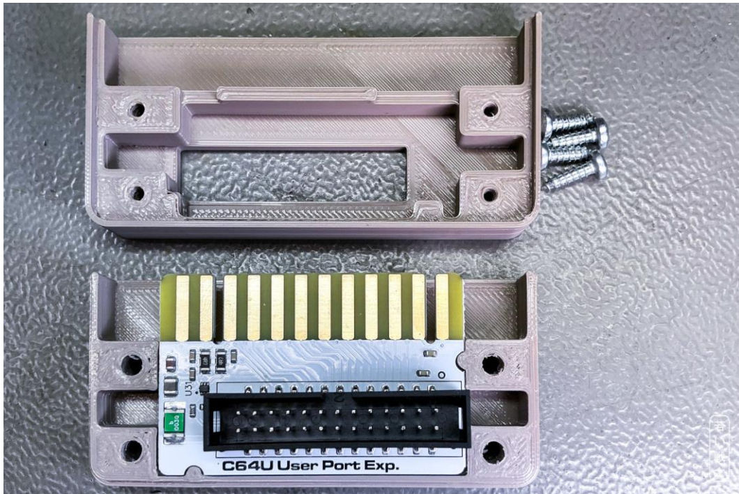
Figure 4: User Port PCB inside the open case
