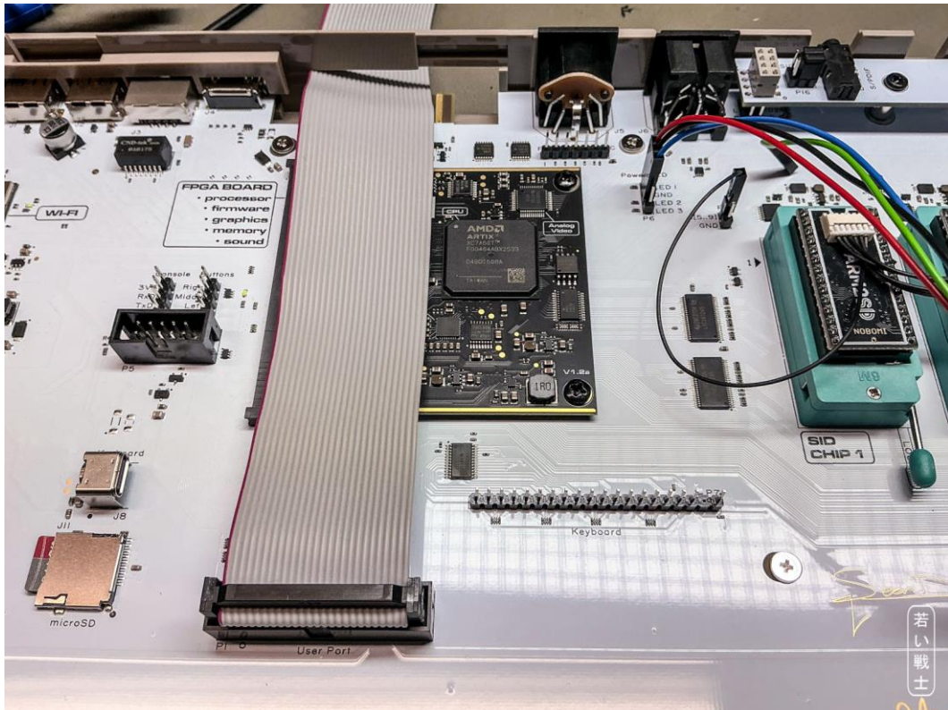
Figure 1: User Port ribbon cable inside a C64 Ultimate
